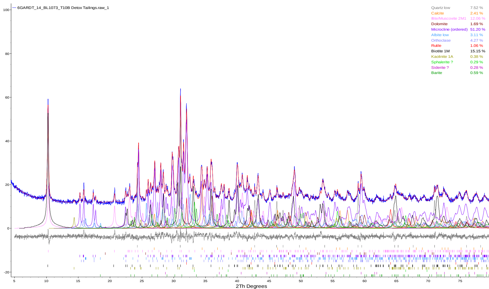
Figure 6. Rietveld refinement plot of sample Global ARD Testing Services #14: BL1073-T10B Detox Tailings (blue line - observed intensity at each step; red line - calculated pattern; solid grey line below - difference between observed and calculated intensities; vertical bars - positions of all Bragg reflections). Coloured lines are individual diffraction patterns of all phases.
