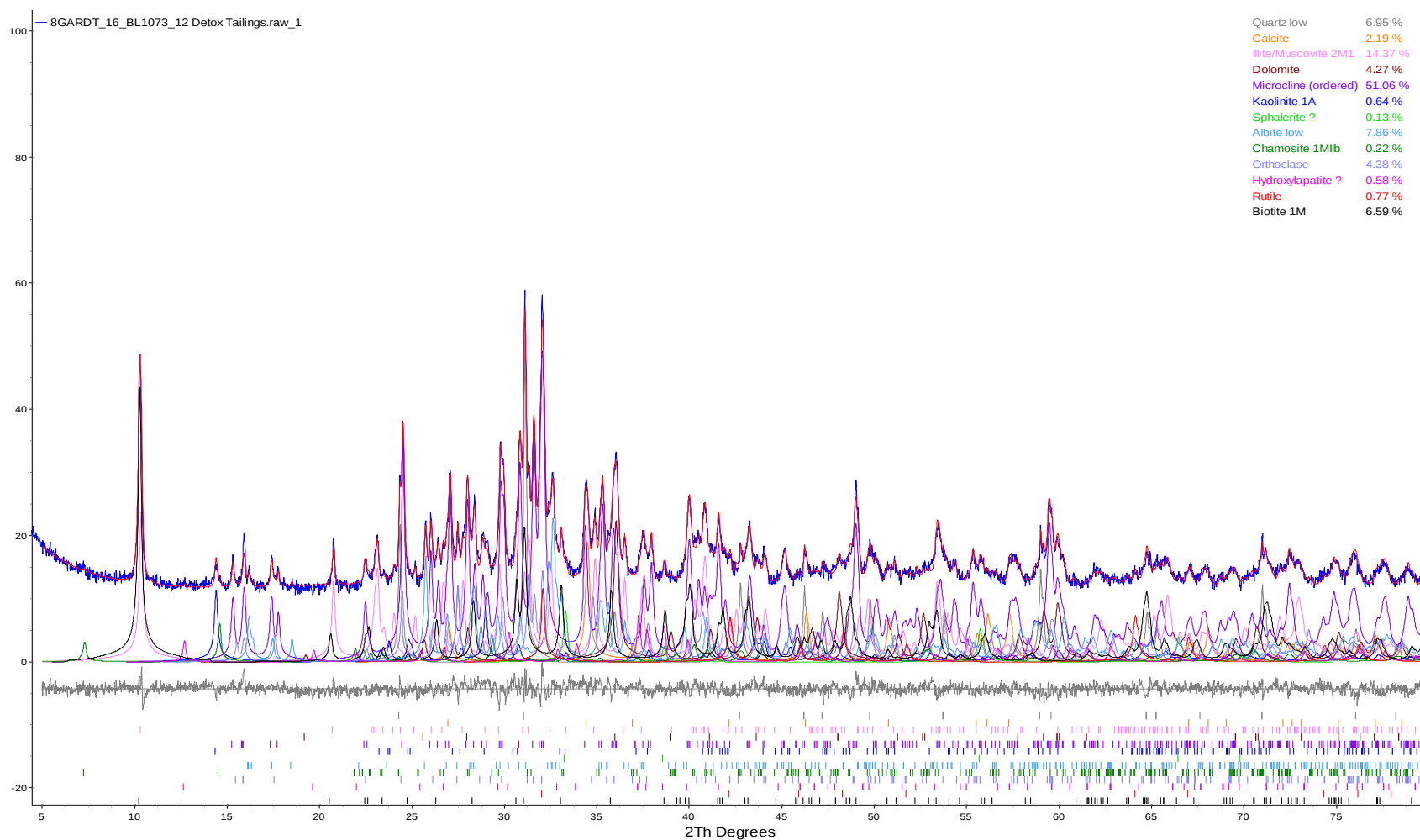
Figure 8. Rietveld refinement plot of sample Global ARD Testing Services #16: BL1073-12 Detox Tailings (blue line - observed intensity at each step; red line - calculated pattern; solid grey line below - difference between observed and calculated intensities; vertical bars - positions of all Bragg reflections). Coloured lines are individual diffraction patterns of all phases.
