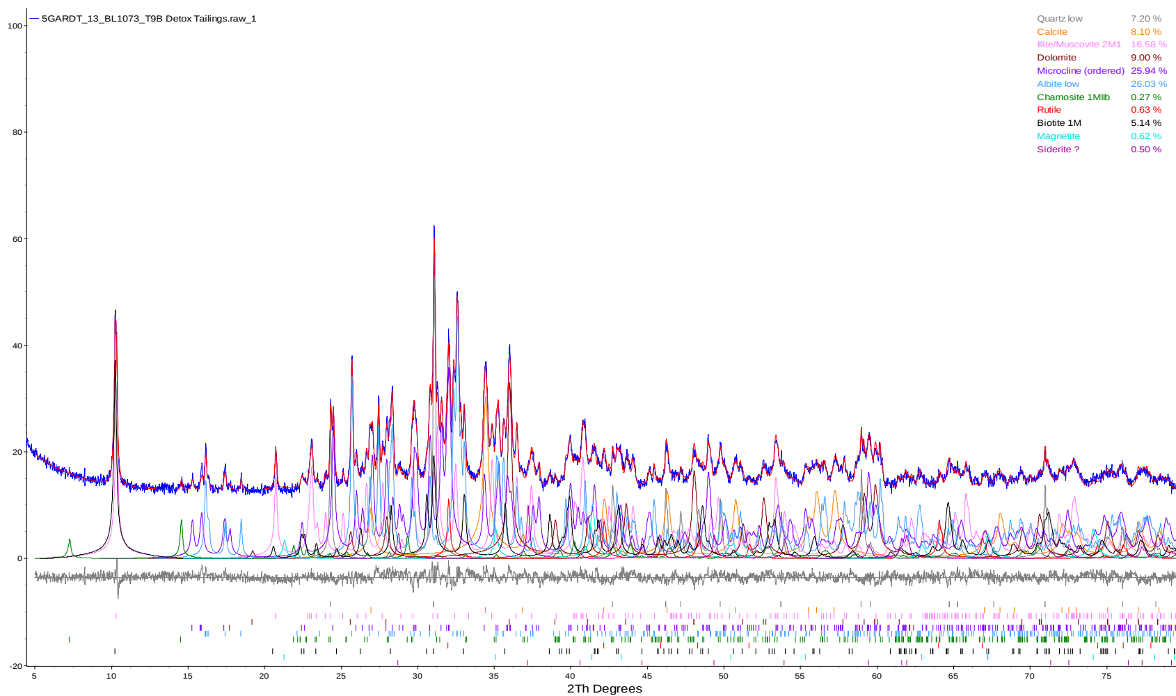
Figure 5. Rietveld refinement plot of sample Global ARD Testing Services #13: BL1073_T9B Detox Tailings (blue line - observed intensity at each step; red line - calculated pattern; solid grey line below - difference between observed and calculated intensities; vertical bars - positions of all Bragg reflections). Coloured lines are individual diffraction patterns of all phases.
